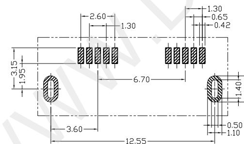
RECOMMEND PCB LAYOUT(TOP VIEW) GENERAL TOLERANCE \pm 0.05
